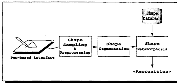
Figure 1: Metamorphosis-based shape recognition system.
