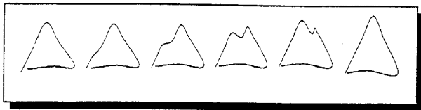
Figure 5: Chaotic metamorphosis of a triangle to a similar triangle.
