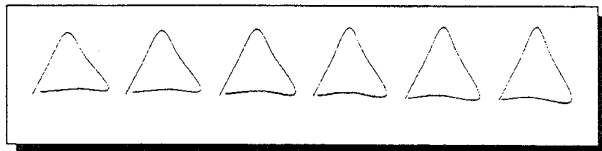
Figure 4: Non-chaotic metamorphosis of a triangle to a similar triangle.
